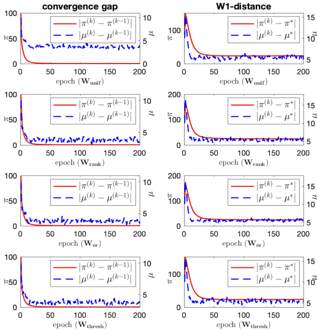
Figure 1. Algorithm performance (Flocking-Graphon)
